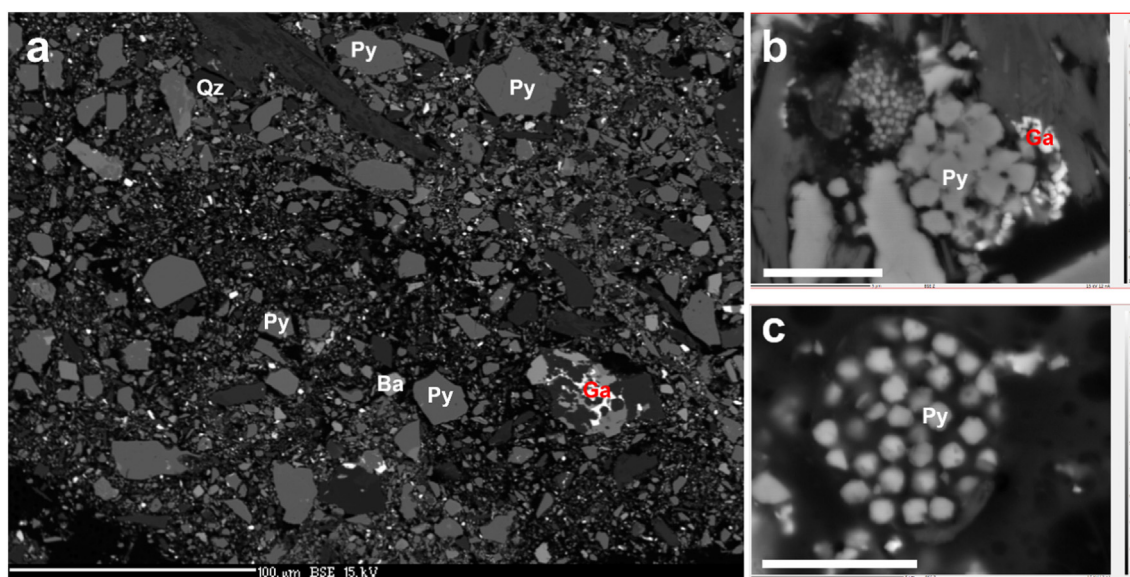
Fig. 6. EPMA-SEM of tailings concentrate (a) and tailings concentrate after bioleaching (b). Qz: quartz, Py: pyrite, Ba: barite, Ga: galena. Bar in b and c represents 5 µm.
